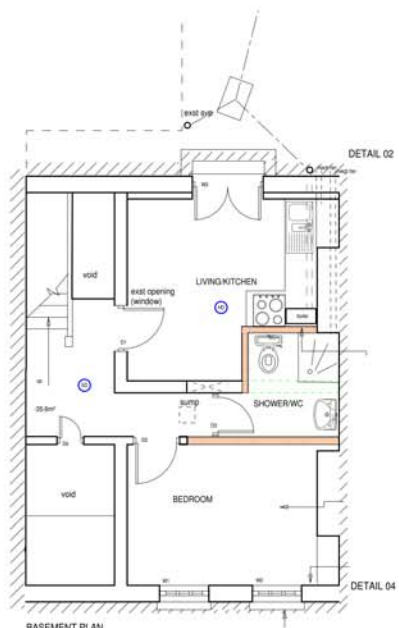
BASEMENT PLAN 1 Bedroom Unit
