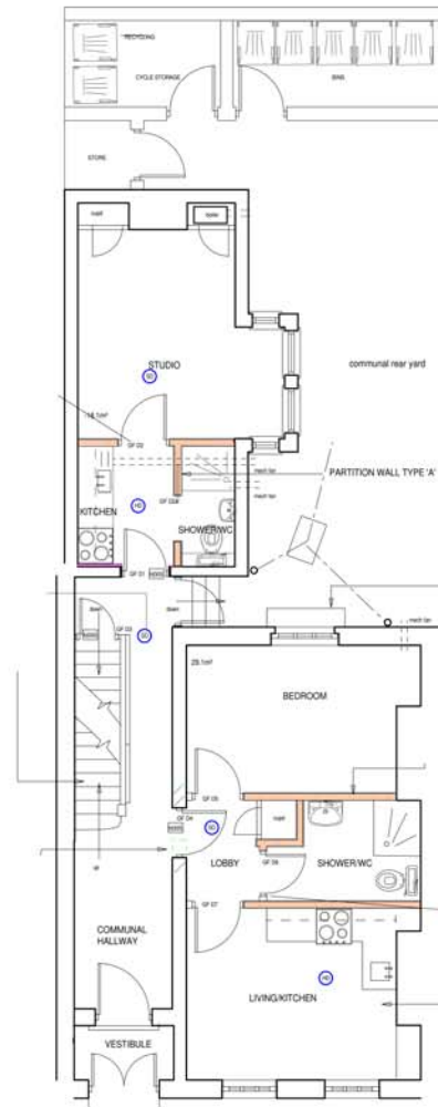
GROUND FLOOR PLAN 1no. Studio Unit 1no. 1 Bedroom Unit
